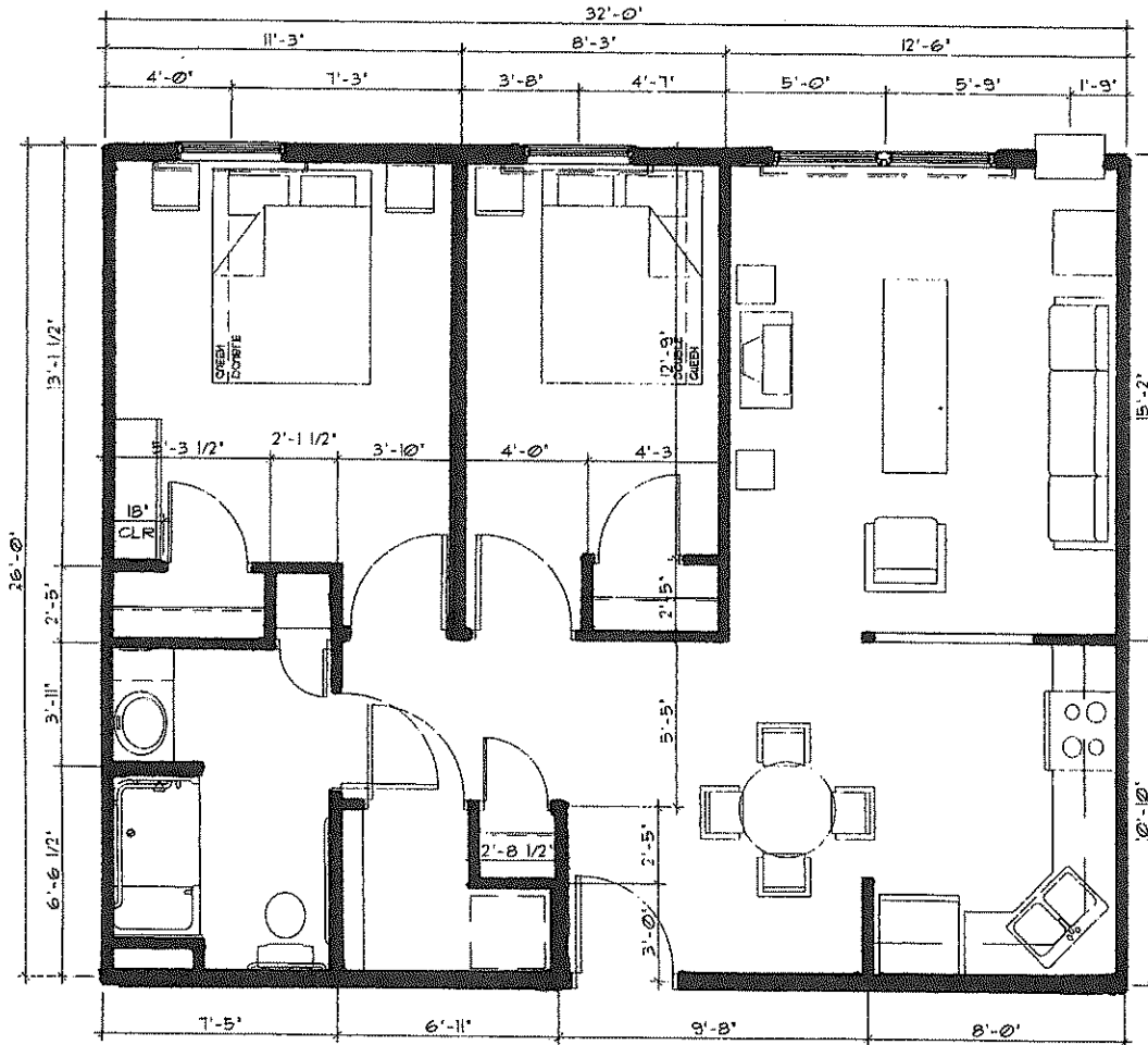
2 A-4 TYPICAL TWO BEDROOM UNIT SCALE: 1/4"=1'-0"
